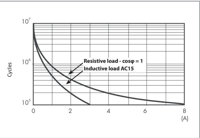
F 40.2 - Electrical life (AC) v contact current Type 40.52
