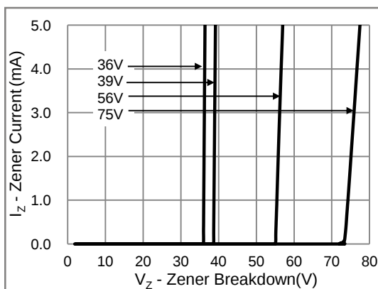
Fig.5 Typical Zener Breakdown
