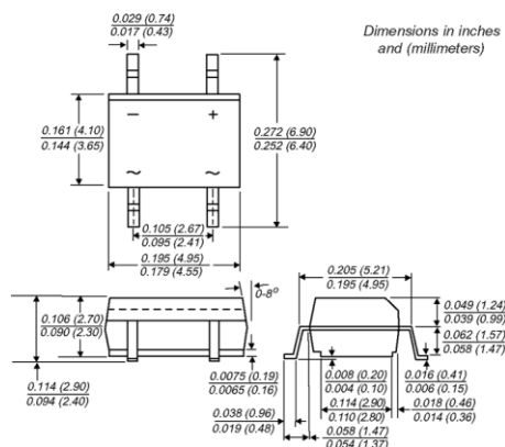
TO-269AA (MBS)
