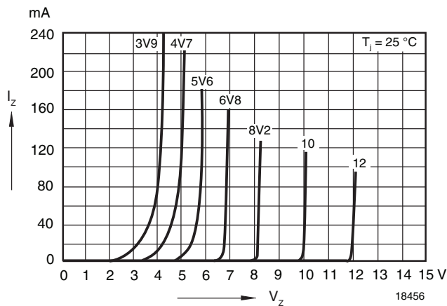
Fig. 3 - Typical Breakdown Characteristics
