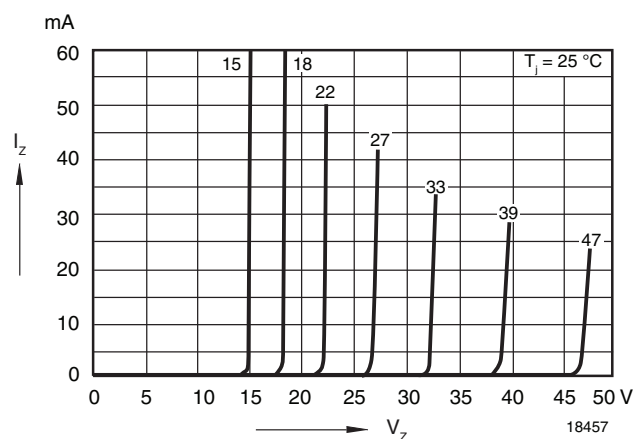
Fig. 4 - Typical Breakdown Characteristics
