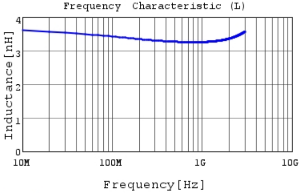
LQP03TN3N3B02 L
