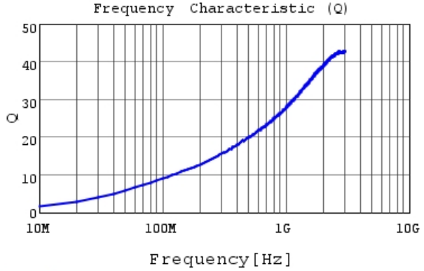
LQP03TN3N3B02 Q
