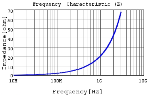
LQP03TN3N3B02 |Z|
