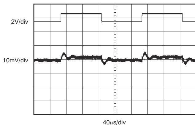
Figure 5-31. Step Response
