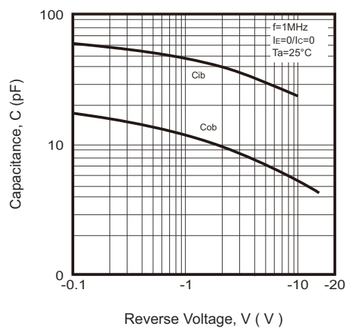
Fig.7 - C_{ob}/C_{ib} — V_{CB}/V_{EB}
