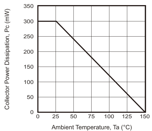
Fig.8 - P_C — T_a
