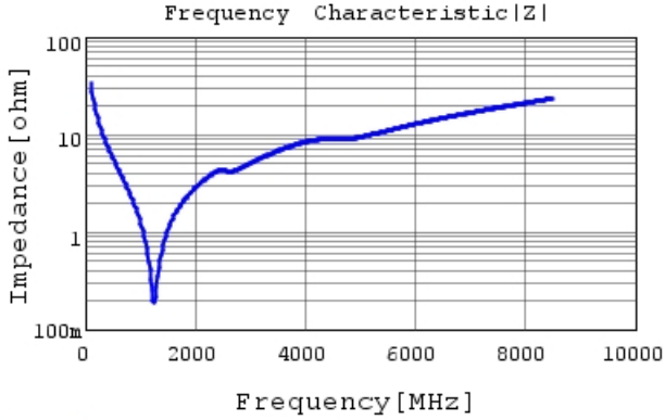
GRT1555C1H470JA02 |Z| DC0V, 25degC
