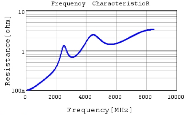
GRT1555C1H470JA02 R DC0V, 25degC
