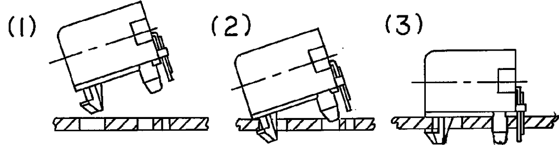
MOUNTING PROCEDURE
