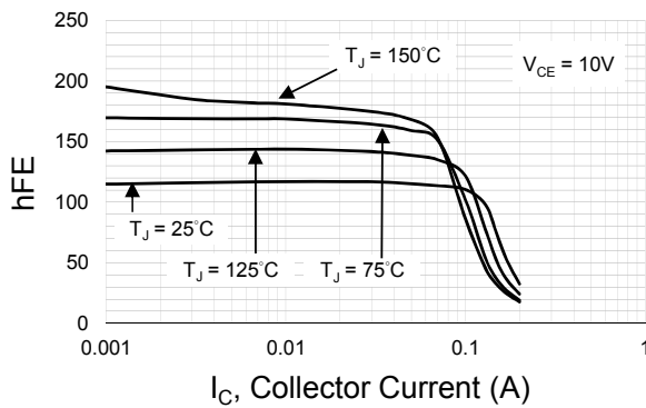
Fig.3 Typical DC Current Gain vs Collector Current
