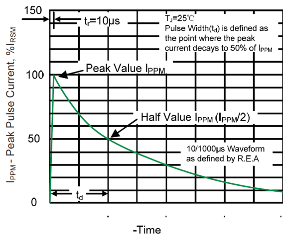
Figure 3. Pulse Waveform
