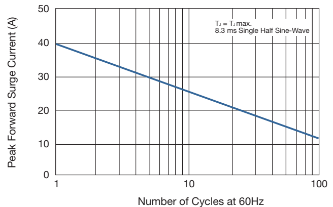
FIG 2. MAXIMUM NON-REPETITIVE
