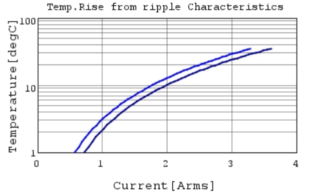
GRM155C81A225KE11 Temp.rise — 500kHz
