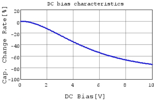
GRM155C81A225KE11 C-DC bias capchange, 25.0c
