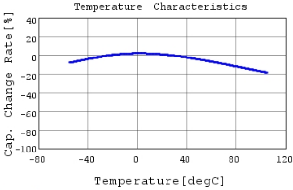
GRM155C81A225KE11 C-Temp. capchange, DC0.0V,
